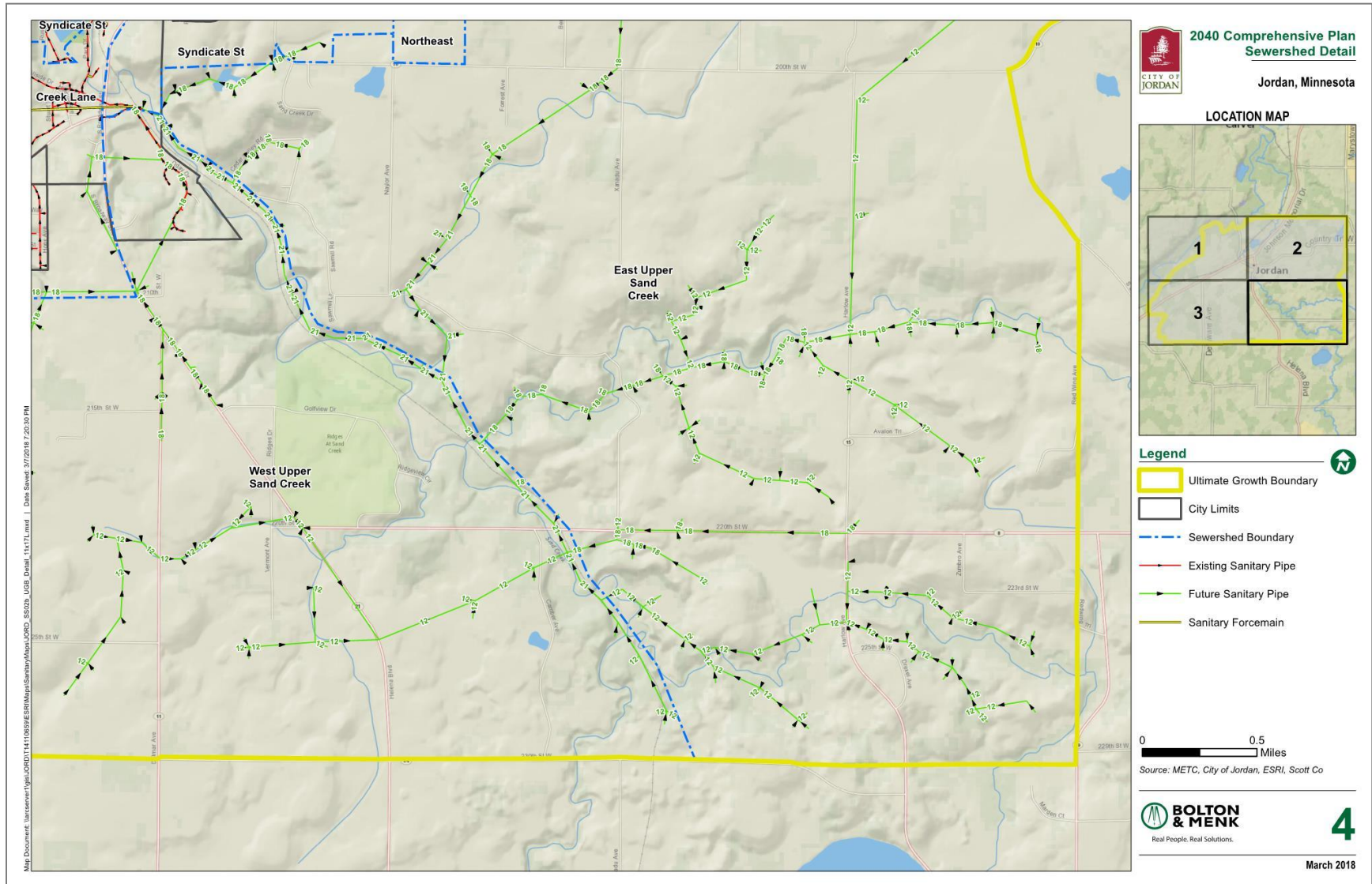
Map 4-6: SEWERSHED DETAIL
